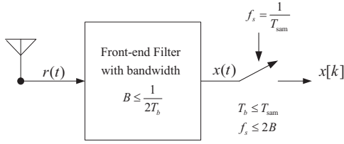
Fig. 1. The receiver's analog front-end. The output of the front-end filter is sampled at rate 1/T_{\text{sam}} , which is smaller than its Nyquist sampling rate 2B .
